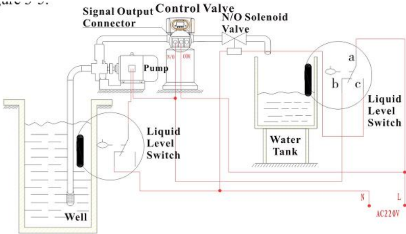
Figure 3-5 Wiring of Liquid Level Controlling Inlet Pump
