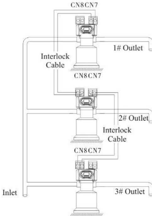
Figure 3-10 Interlock System
