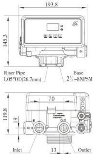
F71Q1 structure chart:
