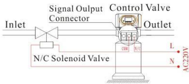
Figure 3-2 Wiring of Solenoid Valve on Inlet
