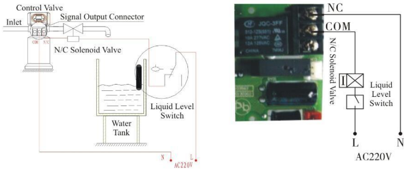
Figure 3-1 Wiring of Solenoid Valve on Outlet
