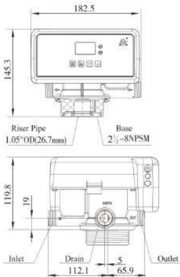
F71Q1 structure chart:
