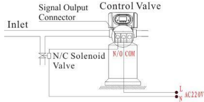
Figure 3-3 Wiring of Pressure Relief Connector
