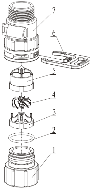
5447018 Flow Meter
