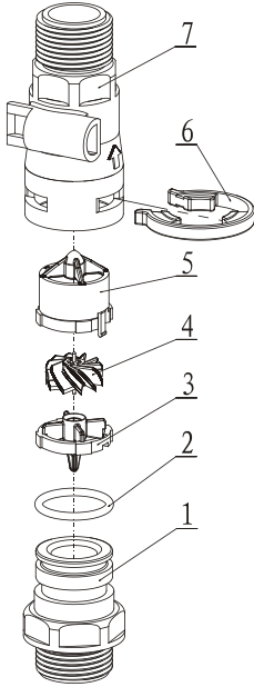
5447020 Flow Meter
