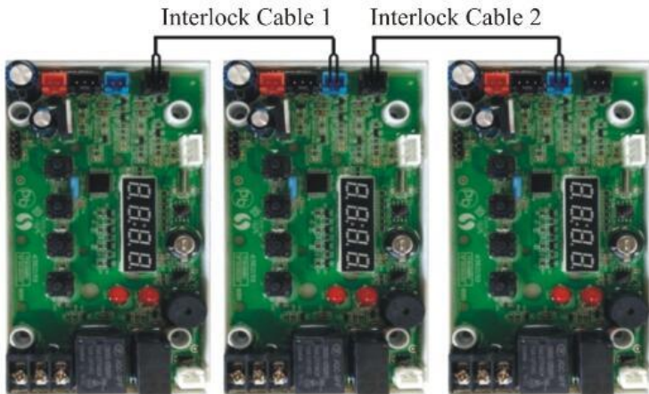
Figure 3-9 Interlock
